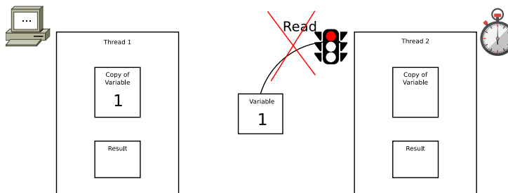
Figure 122: How mutex works (3/8)
